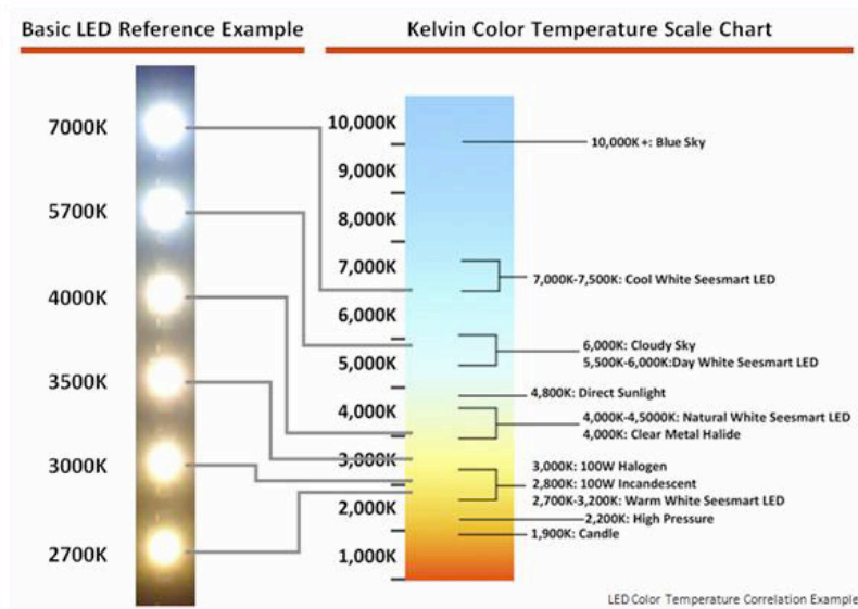
Figure 13: Color Temperature Scale
